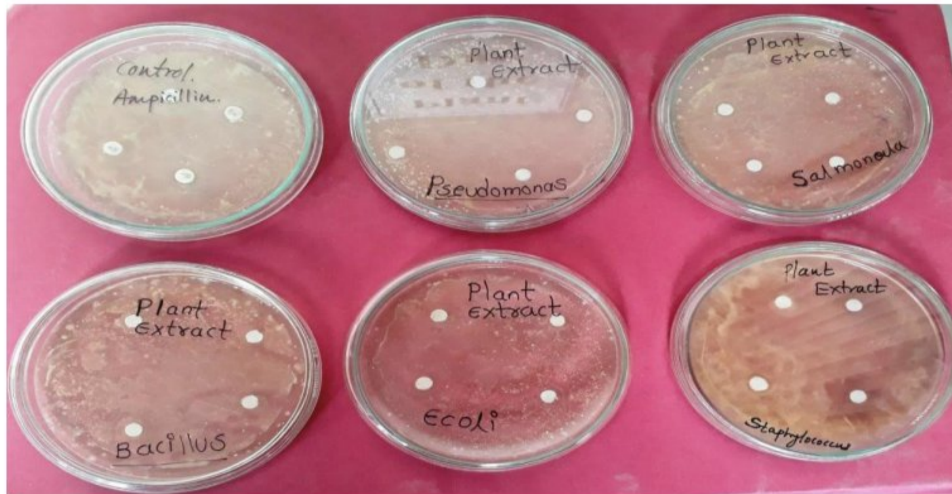
Plate 3: Antibacterial activity of silver nanoparticles against Escherichia coli , Bacillus subtilis , Salmonella abony , Staphylococcus aureus and Pseudomonas aeruginosa .
