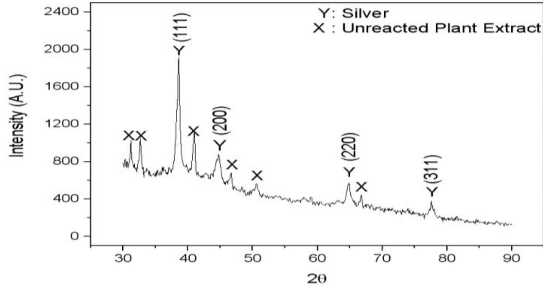
Fig. 3: XRD pattern of AgNPs.
