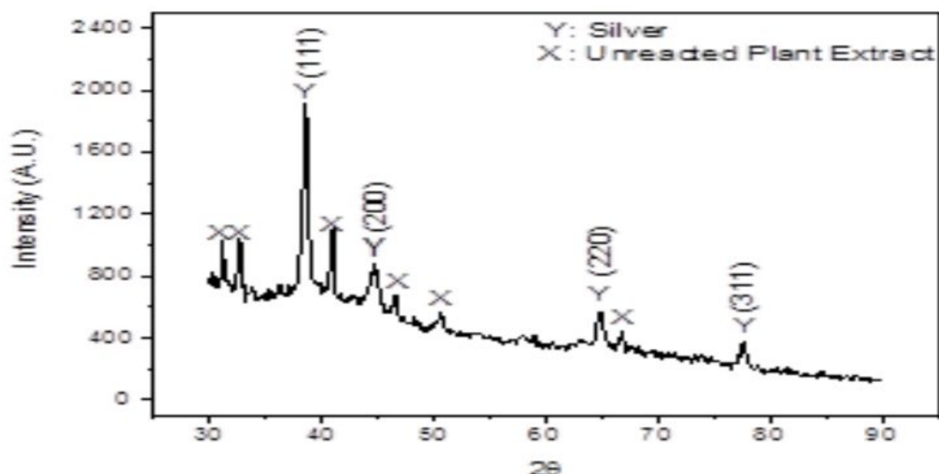
Fig. 3: XRD pattern of AgNPs.
